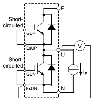
Gate-emitter short-circuited GUP-EsUP, GUN-EsUN, GVP-EsVP, GVN-EsVN, GWP-EsWP, GWN-EsWN, GB-EsB
