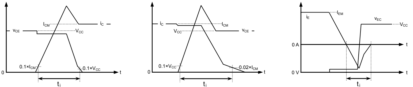
IGBT Turn-on switching energy IGBT Turn-off switching energy DIODE Reverse recovery energy Turn-on / Turn-off switching energy and Reverse recovery energy test waveforms (Integral time instruction drawing)
