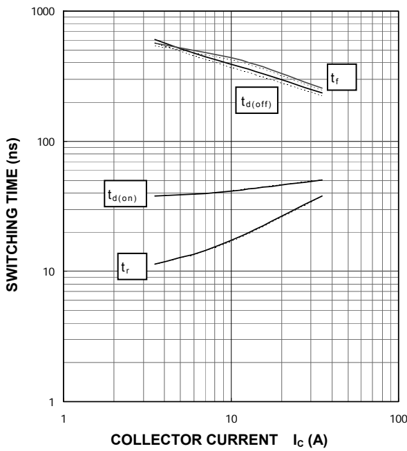
HALF-BRIDGE SWITCHING CHARACTERISTICS (TYPICAL) V_{CC}=600\text{ V} , V_{GE}=\pm 15\text{ V} , R_G=18\ \Omega , —: T_j=150\text{ }^\circ\text{C} , - - - -: T_j=125\text{ }^\circ\text{C}
