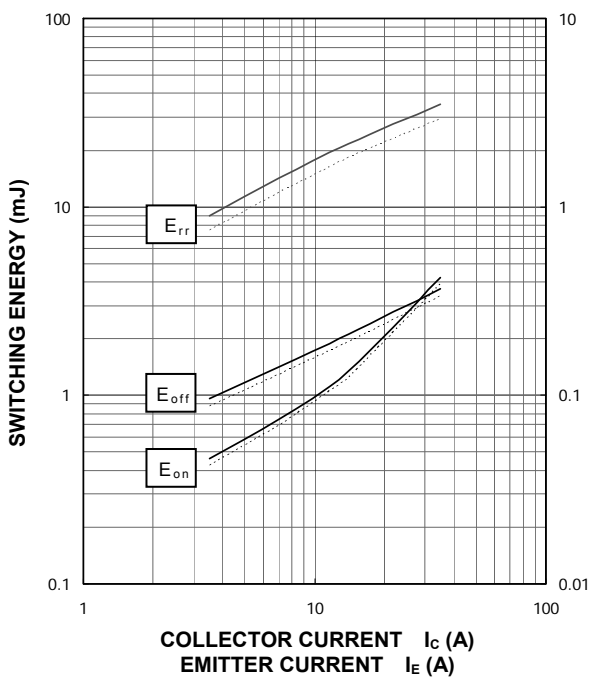
HALF-BRIDGE SWITCHING CHARACTERISTICS (TYPICAL) V_{CC}=600\text{ V} , V_{GE}=\pm 15\text{ V} , R_G=18\ \Omega , —: T_j=150\text{ }^\circ\text{C} , - - - -: T_j=125\text{ }^\circ\text{C}
