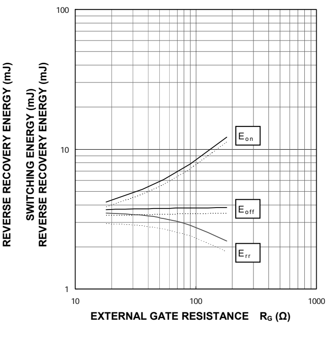
HALF-BRIDGE SWITCHING CHARACTERISTICS (TYPICAL) V_{CC}=600\text{ V} , V_{GE}=\pm 15\text{ V} , I_C=35\text{ A} , —: T_j=150\text{ }^\circ\text{C} , - - - -: T_j=125\text{ }^\circ\text{C}
