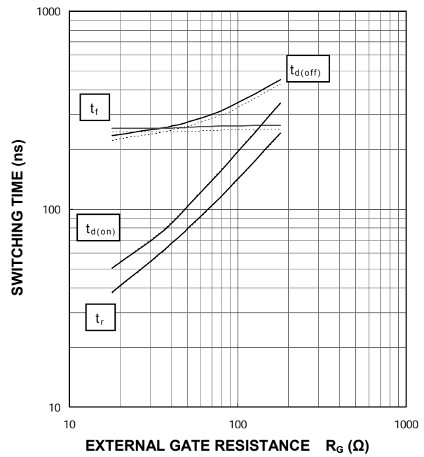
HALF-BRIDGE SWITCHING CHARACTERISTICS (TYPICAL) V_{CC}=600\text{ V} , V_{GE}=\pm 15\text{ V} , I_C=35\text{ A} , —: T_j=150\text{ }^\circ\text{C} , - - - -: T_j=125\text{ }^\circ\text{C}
