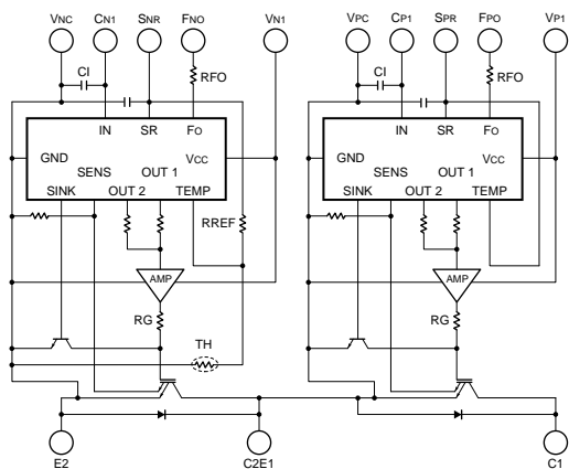
Outline Drawing and Circuit Diagram
