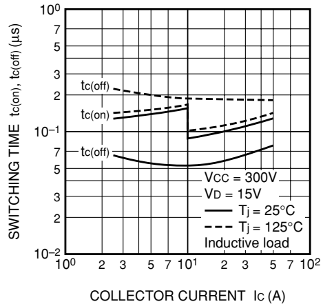
SWITCHING TIME CHARACTERISTICS (Lower Arm - TYPICAL)
