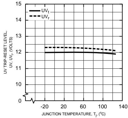
CONTROL SUPPLY VOLTAGE TRIP-RESET LEVEL TEMPERATURE DEPENDANCY (TYPICAL)
