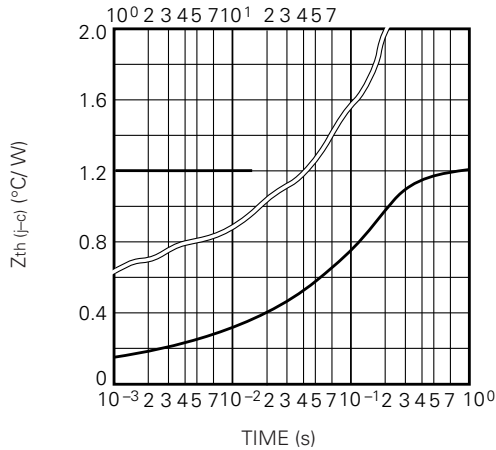
TRANSIENT THERMAL IMPEDANCE CHARACTERISTIC (DIODE)
